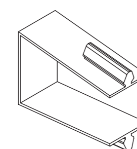
Georgian Bar Clip 28mm Art. No. 200344
